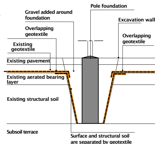
Restoration when laying foundation in existing structural soil.
